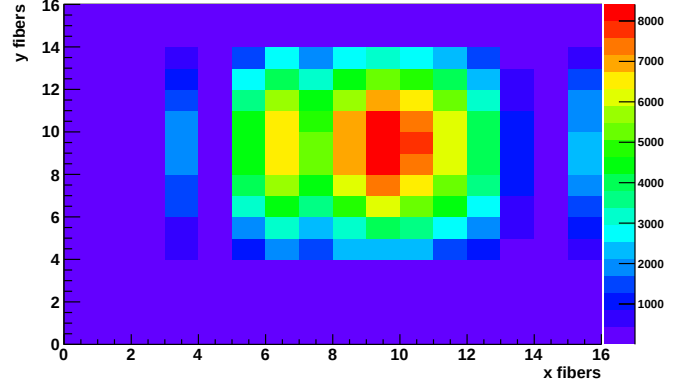
Fig. 13. Beam profile, measured with 25 MeV protons.
