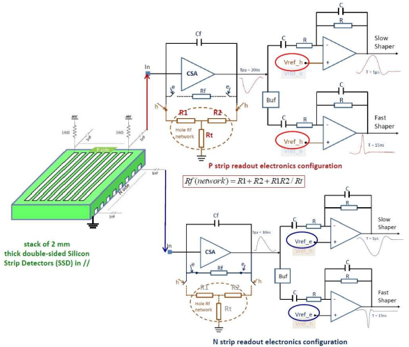
Fig. 7. Scheme of readout electronics [35] for the SSD.
