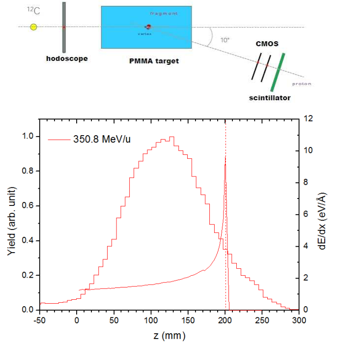
Fig. 10. Experimental configuration at HIT (top) and measured reconstructed vertices in comparison to the corresponding stopping power (bottom).
