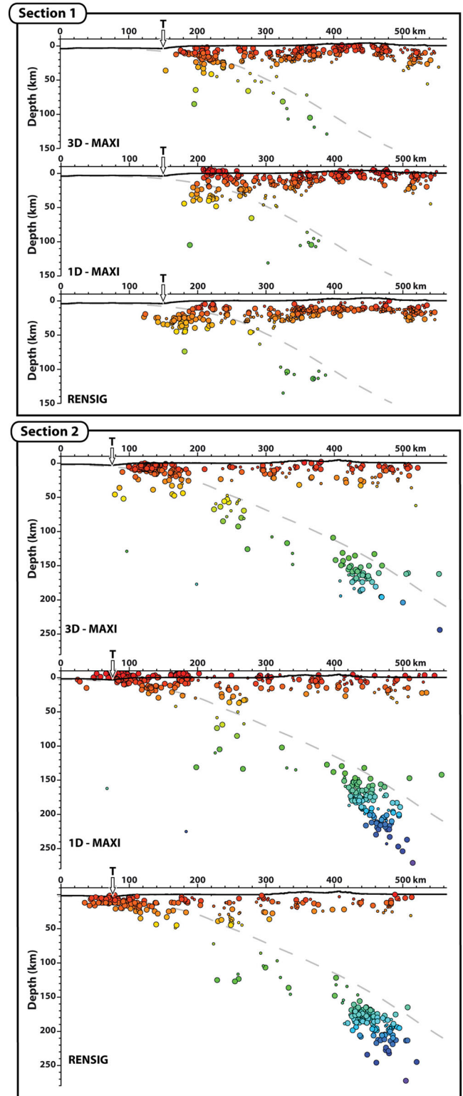
Figure 10. Seismicity cross-sections comparing earthquake location resulting from three different procedures (location on Fig. 9). See Fig. 9 for explanations about 3-D- MAXI , 1-D- MAXI and RENSIG procedures. The grey dash line marks an eventual position of the Nazca Plate top and serves as spatial reference.
