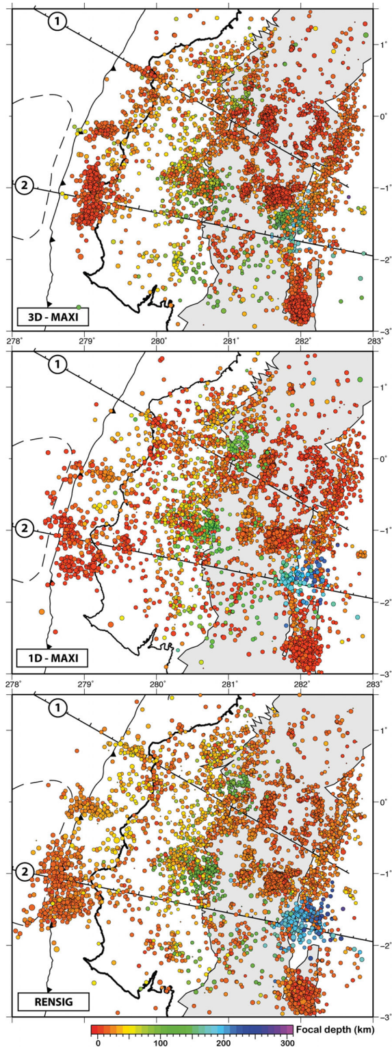
Figure 9. Seismicity map comparing earthquake location resulting from three different procedures. 3-D- MAXI refers to the catalogue resulting from earthquake location using: a selection of RENSIG stations, P arrivals, 3-DVM, and the MAXI technique (see text for more details). 1-D- MAXI : identical procedure within a 1-D-layered model (from the RENSIG ). RENSIG refers to the whole network, P - and S -waves arrivals, 1-D-layered model (see Table 3) and FASTHYPO (Herrmann 1979). The traces of the Carnegie Ridge (dashed line), the trench (bold line and triangles) and the Andean Chain (in grey) are marked for references. 1 and 2 identify the cross-section shown on Fig. 10.
