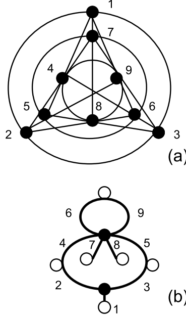
Fig. 8. The Hesse configuration (a) and an associated genus-zero dessin (b).
