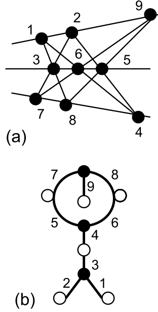
Fig. 9. The Pappus configuration (a) and a stabilizing dessin (b).
