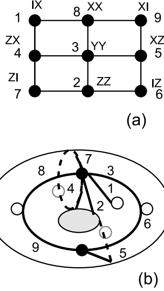
Fig. 7. A 3 \times 3 grid with points labeled by two-qubit observables ( aka a Mermin magic square) (a) and a stabilizing dessin drawn on a torus (b).
