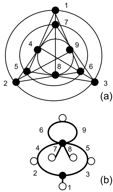
Figure 8. The Hesse configuration (a) and an associated genus-zero dessin (b).
