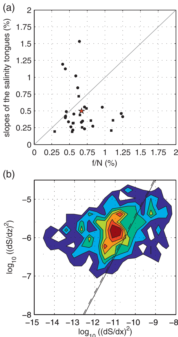
FIG. 12. (a) Comparison between f/N (calculated at 100-m depth) and slopes of the salinity structures (estimated from the local salinity minima and maxima at 120 and 80 m). Squares (circles) mark values from saline (fresh)water anomalies. The red star marks the center of mass of the distribution. (b) Probability distribution function of (\partial S/\partial z)^2 and (\partial S/\partial x)^2 at 100 m. The black line represents the slope (N/f)^2 (calculated at 100-m depth) and the dashed line represents the slope of the median value of (\partial S/\partial z)^2/(\partial S/\partial x)^2 .
