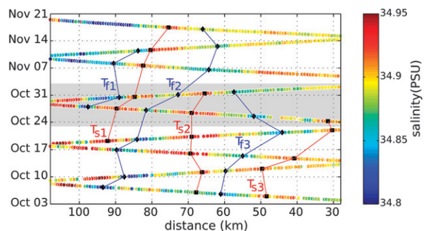
FIG. 8. Hovmöller diagram of salinity at 120 m. Black squares and diamonds indicate the position of local maxima and minima, respectively, representative of each salinity features observed on the vertical sections. Blue (red) lines represent the displacement of the anomalously fresh (saline) features with time. The gray area highlights the period including the glider sections #5 and #6 presented in Fig. 7.
