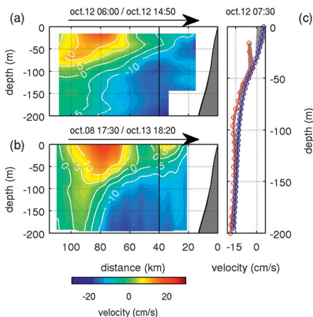
FIG. 3. (a) ADCP current and (b) absolute geostrophic current from glider section #2, perpendicular to the glider section. The meeting point between the glider and the ship is indicated by a vertical black line. (c) Velocity profiles from ADCP data (red line) and from glider data (blue line) at the meeting point. Profiles around the meeting point (within 10 km and 15 h for the glider and 10 km and 1 h for the R/V Olaya ) are indicated in gray.
