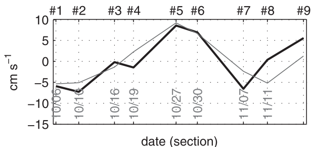
FIG. 4. Surface geostrophic velocity anomaly at 14.27^{\circ}\text{S} , 77^{\circ}\text{W} derived from AVISO (thin gray line) and from the glider data (bold black line). Glider surface velocity anomaly was averaged around the AVISO data point ( \pm 20 km, 0–10-m depth).
