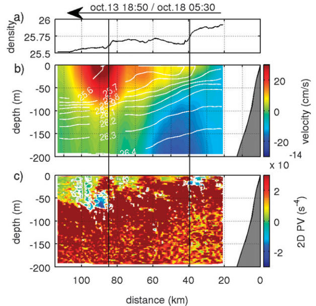
FIG. 10. (a) Cross-shore surface density profile, (b) absolute geostrophic velocity perpendicular to glider section #3 (color coded, \text{cm s}^{-1} ). Smoothed density contours are indicated by white lines. (c) 2D potential vorticity q (color coded, \text{s}^{-4} ) from glider section #3 with white contour corresponding to q = 0 \text{ s}^{-4} . Vertical black lines mark the position of the most pronounced surface density fronts.
