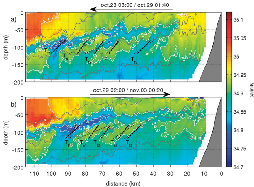
FIG. 7. Salinity from glider section (a) #5 and (b) #6 (color coded); salinity contours (white) and density contours (gray) are overlaid. The slopes of the salinity structures are marked by thin dashed lines (calculated from the minimum of salinity at 120 m and 80-m depth). Bold dashed lines mark f/N slopes, with N calculated at 100-m depth.
