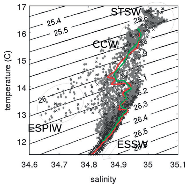
FIG. 2. The \Theta – S diagram from glider section 2 data (diamonds) and from R/V Olaya CTD data along the glider track (crosses). Green and red lines indicate the closest profiles (3.8 km and 1h 30 min) from the glider and the ship, respectively.
