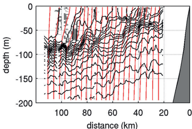
FIG. 11. Absolute momentum surface (red contours, \text{m s}^{-1} ) and density (black contours, \text{kg m}^{-3} ) for glider section #3. Contour intervals are 0.15 \text{ m s}^{-1} for absolute momentum and 5 \times 10^{-2} \text{ kg m}^{-3} for density. Zones of negative PV are marked in gray.
