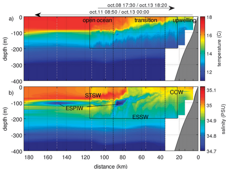
FIG. 5. Vertical sections of (a) potential temperature and (b) salinity carried out from R/V Olaya between 11 and 13 Oct along a section contiguous to the glider sections. The glider section #2 (8–13 Oct) is superimposed in the black rectangle. Three regions (offshore, transition, and coastal) are delimited by black dashed lines. Ship CTD casts are indicated with thin gray-dashed lines.
