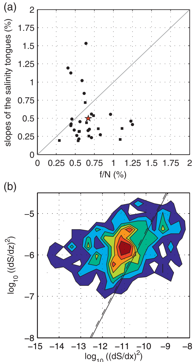
FIG. 12. (a) Comparison between f/N (calculated at 100-m depth) and slopes of the salinity structures (estimated from the local salinity minima and maxima at 120 and 80 m). Squares (circles) mark values from saline (fresh)water anomalies. The red star marks the center of mass of the distribution. (b) Probability distribution function of (\partial S/\partial z)^2 and (\partial S/\partial x)^2 at 100 m. The black line represents the slope (N/f)^2 (calculated at 100-m depth) and the dashed line represents the slope of the median value of (\partial S/\partial z)^2/(\partial S/\partial x)^2 .
