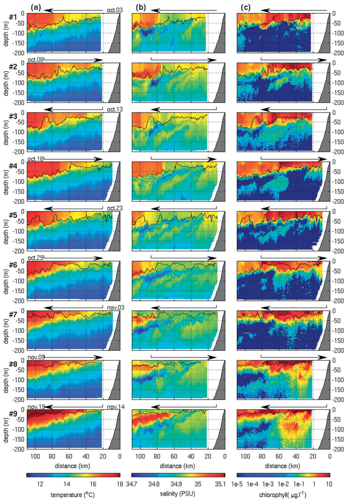
FIG. 6. (a) Potential temperature ( ^{\circ}\text{C} ), (b) salinity (psu), and (c) chlorophyll (concentration, \mu\text{g L}^{-1} ) for all glider sections. The mixed layer depth estimated from a 0.4^{\circ}\text{C} temperature difference criteria is marked by a dark gray line.
