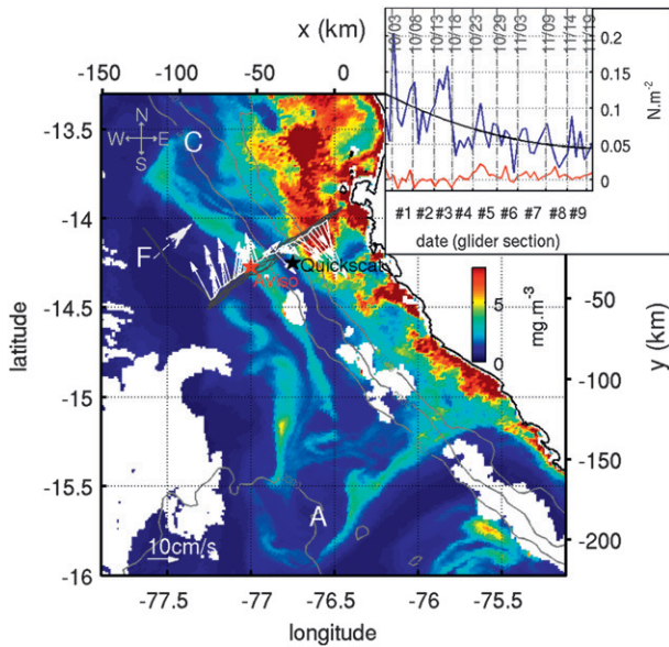
FIG. 1. Surface chlorophyll concentration ( \text{mg m}^{-3} ) from the Moderate Resolution Imaging Spectroradiometer (Modis) (14–16 Nov 2008). Gray lines indicate glider trajectories. The white line indicates the glider trajectory between 14 and 19 Nov (section #9) and white arrows mark 0–200 m depth-averaged water velocities. Location of estimated QuikSCAT windstress is marked by a black star and location of the estimated surface current from AVISO by a red star. Labels denote the location of a cyclonic eddy (C), an anticyclonic eddy (A) and a filament (F). Inset: Quikscat windstress components along (red) and perpendicular (blue) to the glider section.
