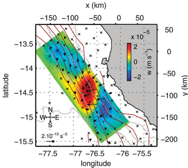
FIG. 9. Vertical velocity at 100 m from the \omega equation. Black arrows represent the \mathbf{Q} vector at 100 m estimated using geostrophic surface velocities derived from altimetry (AVISO) and density from the ship CTDs between 3 and 17 Oct. Black crosses indicate the position of the ship CTDs. Density contours (every 4 \times 10^{-2} \text{ kg m}^{-3} ) are indicated with brown lines. Gray lines indicate the bathymetry.
