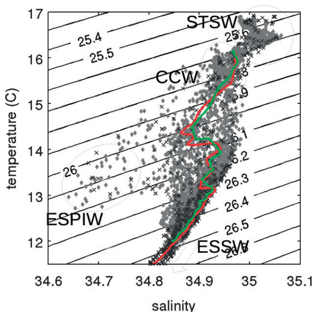
FIG. 2. The \Theta -S diagram from glider section 2 data (diamonds) and from R/V Olaya CTD data along the glider track (crosses). Green and red lines indicate the closest profiles (3.8 km and 1h 30 min) from the glider and the ship, respectively.
