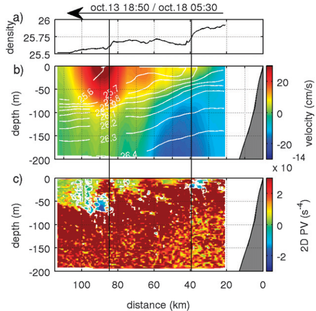
FIG. 10. (a) Cross-shore surface density profile, (b) absolute geostrophic velocity perpendicular to glider section #3 (color coded, \text{cm s}^{-1} ). Smoothed density contours are indicated by white lines. (c) 2D potential vorticity q (color coded, \text{s}^{-4} ) from glider section #3 with white contour corresponding to q = 0 \text{ s}^{-4} . Vertical black lines mark the position of the most pronounced surface density fronts.
