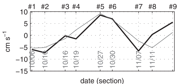
FIG. 4. Surface geostrophic velocity anomaly at 14.27°S, 77°W derived from AVISO (thin gray line) and from the glider data (bold black line). Glider surface velocity anomaly was averaged around the AVISO data point ( \pm 20 km, 0–10-m depth).
