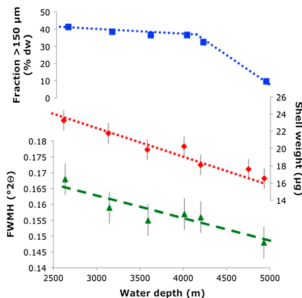
Figure 6. Profiles of three dissolution proxies versus water depth (m): (i) Relative amount of fraction >150 μm (% dry weight) (top panel, blue squares), (ii) shell weight (μg) of G. sacculifer picked from our samples (middle panel, red diamonds), and (iii) full width at half maximum (FWMH, °2θ) of the calcite X-ray diffraction peak (bottom panel, green triangles).
