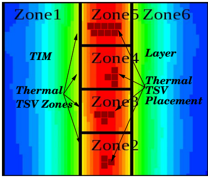
Fig. 5. Special TSV placement Zones at epoxy layer (Re-distribution Layer of Layer 1)
