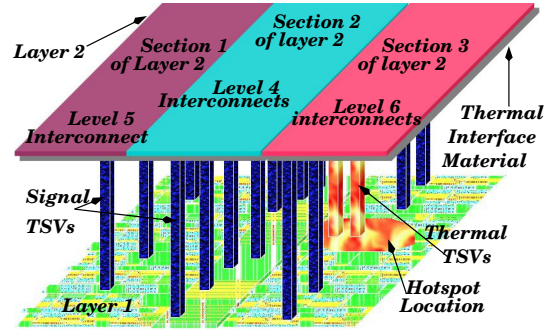
Fig. 3. 2 layer 3D Tree-based FPGA with interconnect levels 4 5 and 6 place in layer 1
