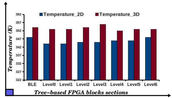
Fig. 6. 3D Thermal analysis of Tree-based interconnect levels and Logic units
