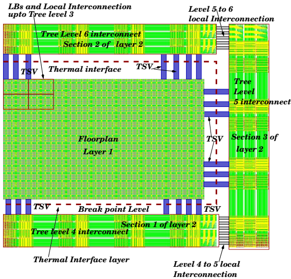
Fig. 2. 3D Tree-based FPGA with break-point between level 3 and 4
