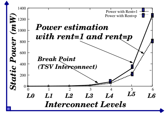
Fig. 4. 3D Tree-based FPGA power estimation: Power consumption at different level with Rent=1 and Rent=p
