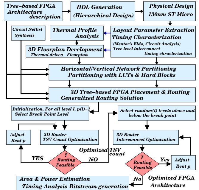
Fig. 1. 3D Tree-based FPGA design optimization methodology
