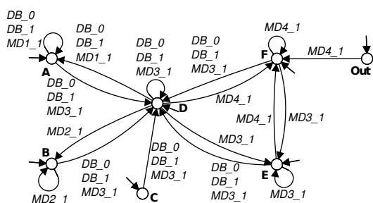
Fig. 2. Detectable Motion Automaton DMA
