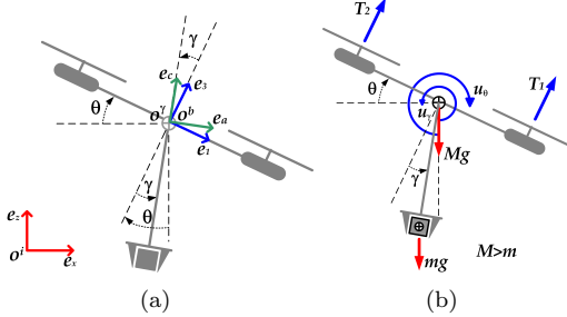
Fig. 1. Freebody diagram: (a) iMAV reference frames and (b) planar freebody diagram
