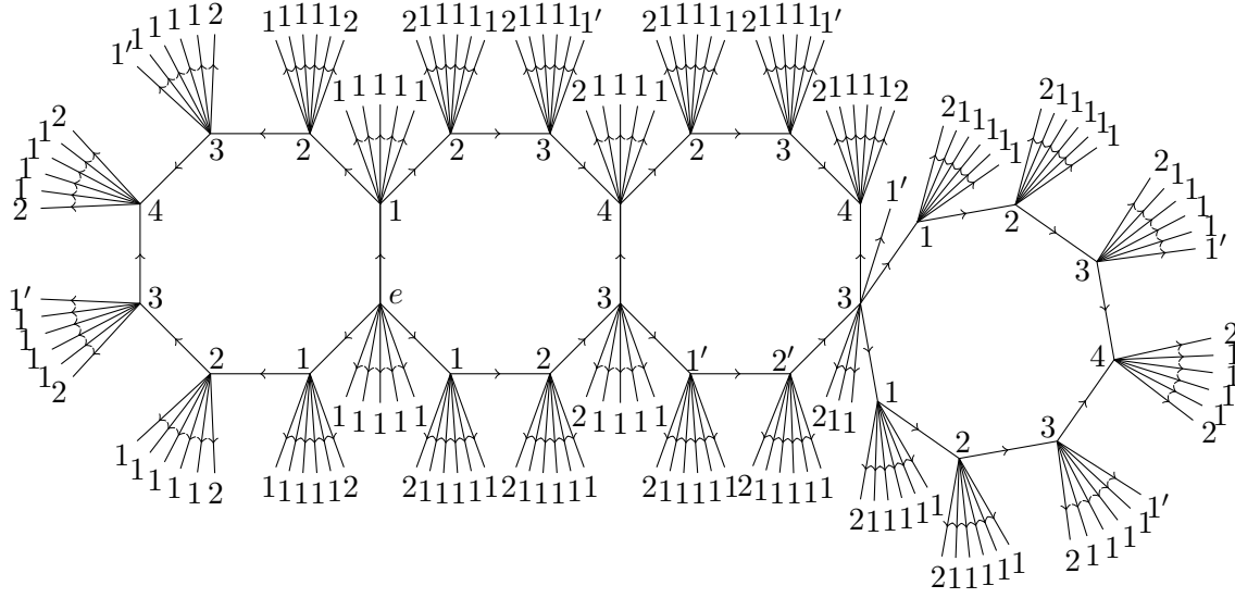
FIGURE 4. Modified Cannon types of the points in (part of) the Cayley graph of \Gamma_2
