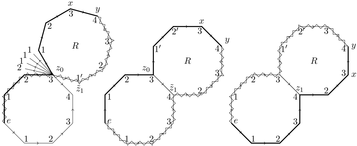
FIGURE 5. Determining the essential type of y from that of x
