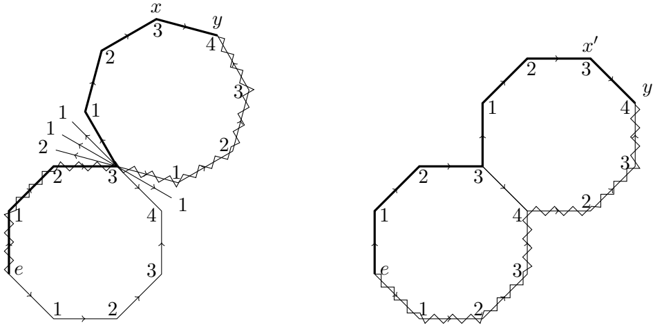
FIGURE 3. x and x' have the same essential type, contrary to y and y' .
