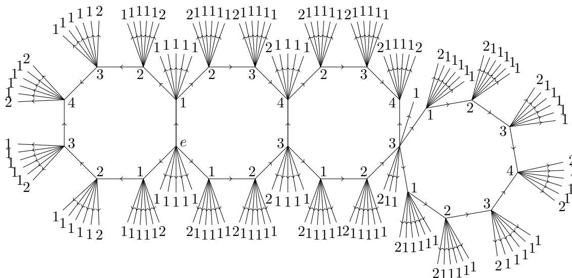
FIGURE 2. Types of the points in (part of) the Cayley graph of \Gamma_2
