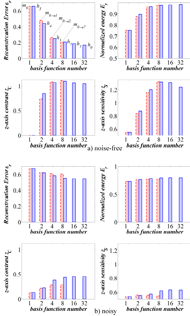
FIG. 5. Performance metrics for both moment-based and Haar-MRA-based reconstructions. The red dash-line bars indicate the metrics of the moments; the blue solid-line bars the metrics of the Haar MRA. C_{max} is set to 10^7 photons. The performance metrics are plotted with respect to the number of BFs used for the reconstruction. The use of 1 BF corresponds to either m_0 or h_5 ; 2 BFs to either m_{0 \rightarrow 1} or h_4 ; 4 BFs to either m_{0 \rightarrow 3} or h_3 ; 8 BFs to either m_{0 \rightarrow 7} or h_2 ; 16 BFs to h_1 ; 32 BFs to h_0 .
