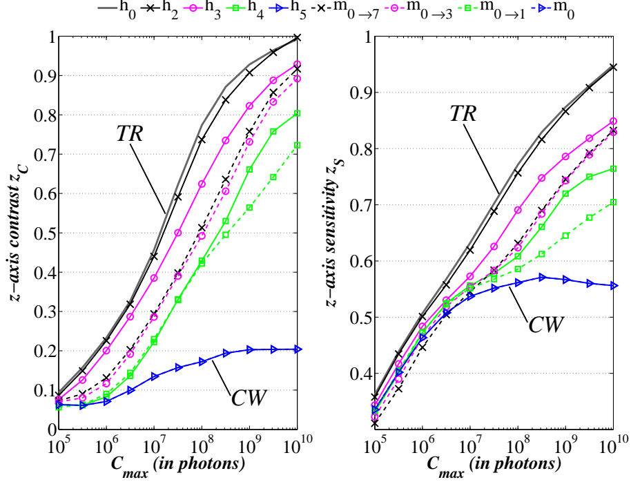
FIG. 7. Evaluation of the z-axis contrast and sensitivity for maximum numbers of detected photons ranging from 10^5 to 10^{10} . The solid lines indicate the use of Haar MRA while the dashed lines indicate the use of moments. The gray solid line without marker is the reference reconstruction obtained from all the TR samples. The number of BFs employed can be 1 (blue line marked with \triangle ), 2 (green line marked with \square ), 4 (pink line marked with \circ ), or 8 (black line marked with \times ).
