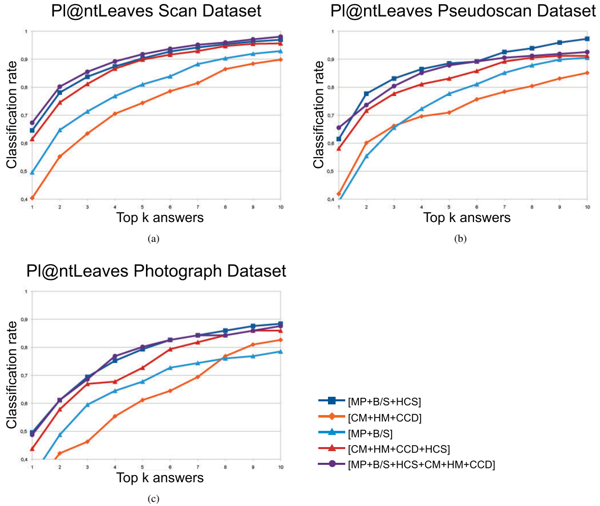
Figure 20: Classification rates on the Pl@ntLeaves Database on scan (a) pseudoscan (b) and photograph (c) images
