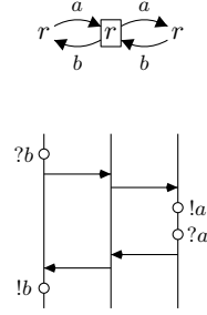
Fig. 7. An MSC over a 1-sphere
