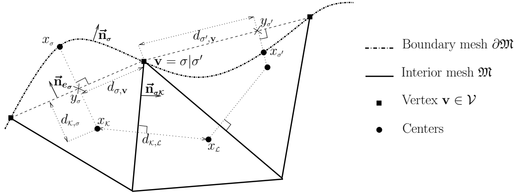
FIGURE 2. Finite volume meshes
