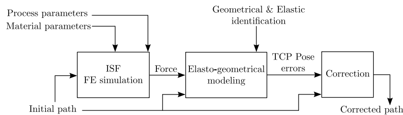
Fig. 13: Post-processor scheme
