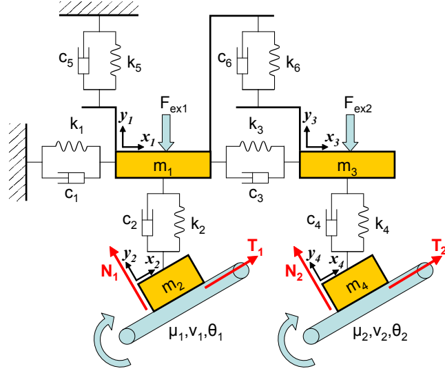
Figure 1: Lumped system considered for calculations.
