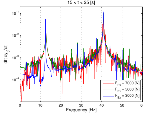
Figure 8: Discrete Fourier Transform of the steady state part of the system response for different external static load.
