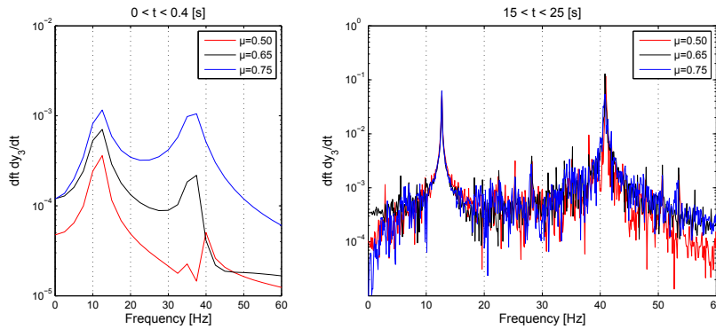
Figure 6: Discrete Fourier Transform of the initial (linear) part and of the final (steady state) part of the system response signal for different friction coefficients
