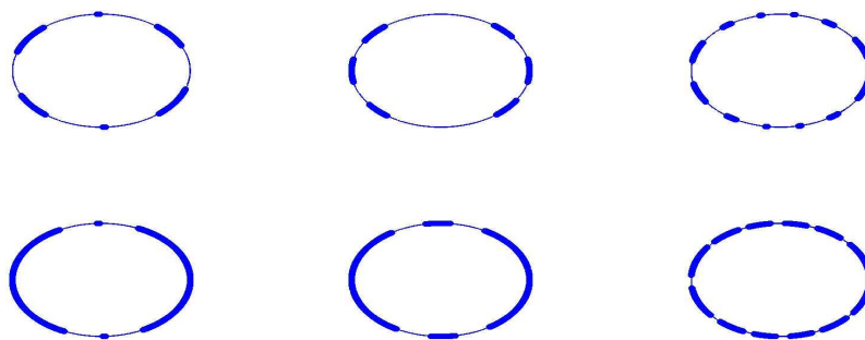
FIGURE 7. The angular sector for 2 and 5 modes ( L = 0.3 , and L = 0.7 )
