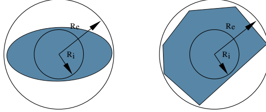
FIGURE 1. Two domains \Omega in dimension 2 for which a_0 \in \overline{\mathcal{U}}_L
