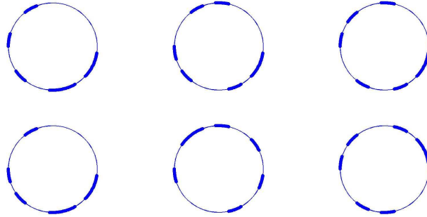
FIGURE 9. The disk for 1, 2 and 5 modes, two examples of solutions ( L=0.3 )
