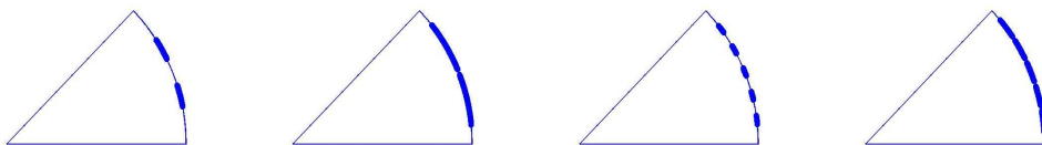
FIGURE 6. The square for 2 and 5 modes ( L = 0.3 , and L = 0.7 )
