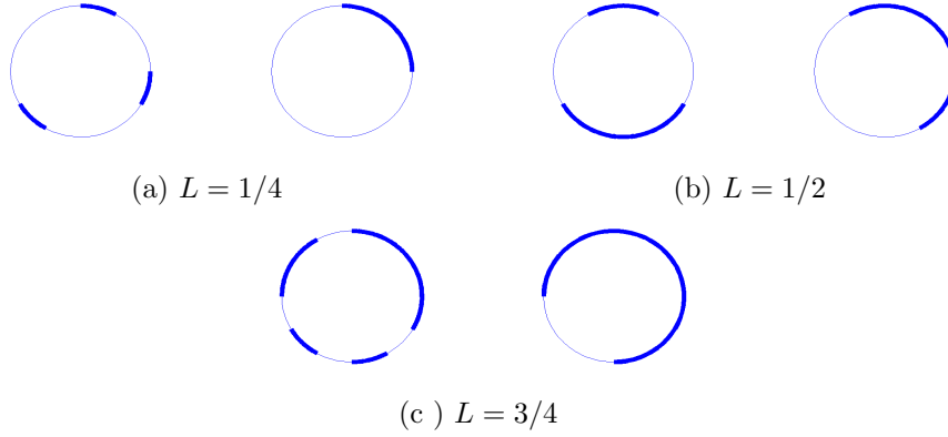
FIGURE 5. \Omega = \{x \in \mathbb{R}^2, \|x\| < 1\} . Some particular solutions for L = 1/4 , L = 1/2 and L = 3/4 .
