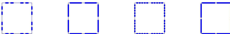
FIGURE 6. The square for 2 and 5 modes ( L = 0.3 , and L = 0.7 )
