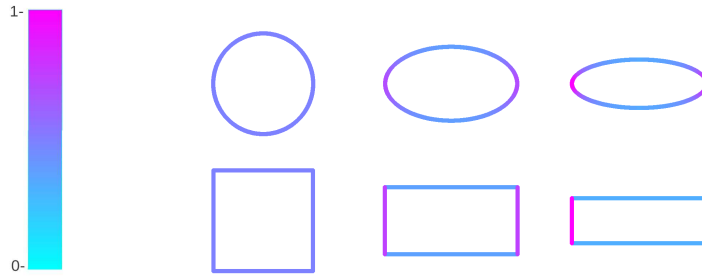
FIGURE 2. Examples of optimal solutions in \overline{\mathcal{U}}_L for several domains \Omega
