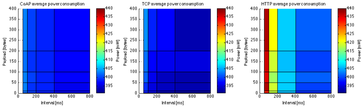
Fig. 2. Measurements of the average power consumption for TCP, HTTP and CoAP on the FLYPORT module
