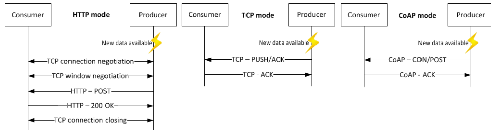
Fig. 3. Packets exchanged in HTTP, CoAP and TCP modes
