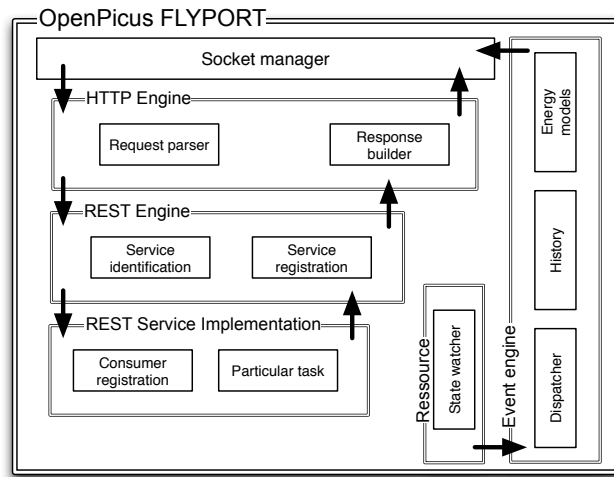
Fig. 4. Architecture deployed on the FLYPORT
