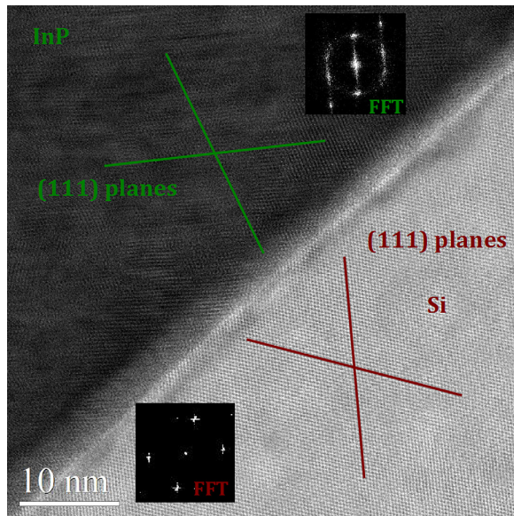
FIG. 3. Atomic-resolution BF-STEM image of the interface between InP and Si below the apex of the indenter. The outlined (1 1 1) and (1 \bar{1} 1) planes of InP and Si reveal that the InP membrane macroscopically rotates during the indentation experiment. Insets show the Fourier transforms of the InP and Si layers.
