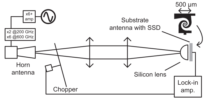
FIG. 7. Setup for free-space measurements of an antenna-coupled InAs SSD at 200 and 600 GHz.
