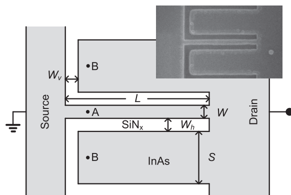
FIG. 1. Schematic view of the geometry of the InAs SSD. Trenches, pictured in white, were etched through the 2DEG of an InAs/Al 80 Ga 20 Sb quantum well. The inset shows a scanning electron microscopy of 100 nm wide etched trenches covered by 25 nm silicon nitride.
