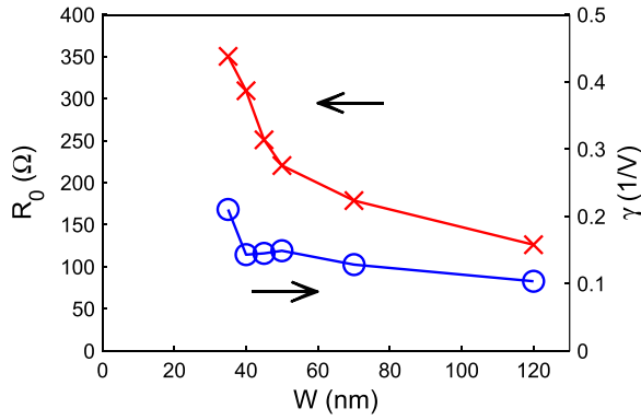
FIG. 5. W -dependence of R_0 (crosses) and \gamma (circles) as found by I-V measurements.
