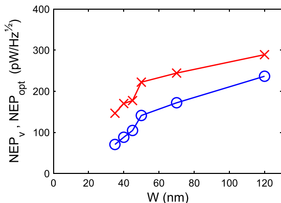
FIG. 6. Measured NEP_v (crosses) and NEP_{opt} (circles) at 50 GHz versus W .
