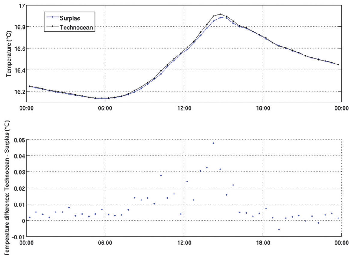
FIG. 3. Comparison of daily cycles (LST) of temperature T_{top} from Technocean drifters with the temperature T_{Surplis} from the Surplis floats: average (top) cycles and (bottom) difference T_{top} - T_{Surplis} over 148 days.
