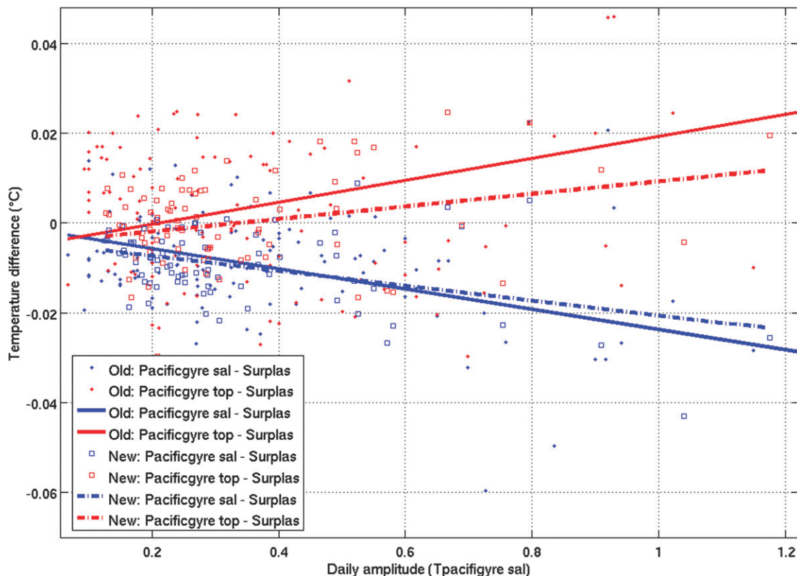
FIG. 5. Scatterplot of difference T_{\text{top}} - T_{\text{Surplas}} (red) and T_{\text{sal}} - T_{\text{Surplas}} (blue) averaged between 1000 and 1600 LST as a function of daily peak-to-peak temperature amplitude from the Pacific Gyre model before 2011 (old, solid lines) and the model since 2011 (new, dashed lines).
