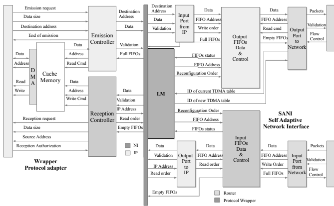
Fig. 3. SANI architecture
