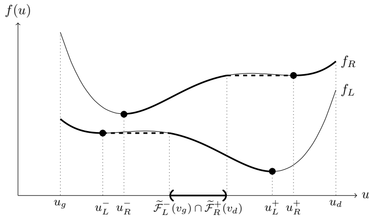
Figure 18: A case where u_g \notin \tilde{\mathcal{F}}_R^+(u_d) , u_d \notin \tilde{\mathcal{F}}_L^-(u_g) , and \tilde{\mathcal{F}}_R^+(u_d) \cap \tilde{\mathcal{F}}_L^-(u_g) \neq \emptyset .
