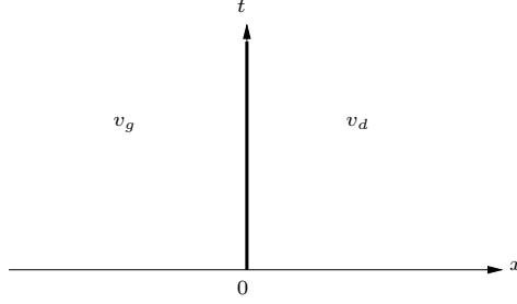
Figure 8: The first type of v-discontinuous solution : a stationary discontinuity.
