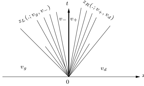
Figure 11: The fourth type of v -discontinuous solution : a L -wave whose right subwave is a rarefaction, followed by a stationary discontinuity, itself followed by a R -wave whose left subwave is a rarefaction.
