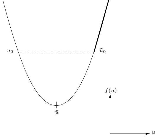
Figure 6: In bold-face, the set \mathcal{F}^+(u_0) , \tilde{u}_0 being excluded.
