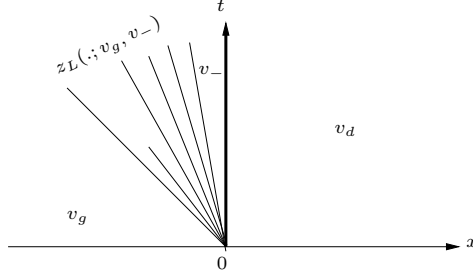
Figure 9: The second type of v -discontinuous solution : a L -wave whose right subwave is a rarefaction, followed by a stationary discontinuity.
