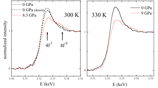
FIG. 1. Ce L_3 -edge XANES of \text{Ce}_{60}\text{Al}_{20}\text{Cu}_{20} metallic glass at 300 K (left) and 330 K (right). Black: ambient, red: high P, dashed: after decompression. Solid arrows mark the |4f^0\rangle (itinerant) and |4f^1\rangle (localized) components.
