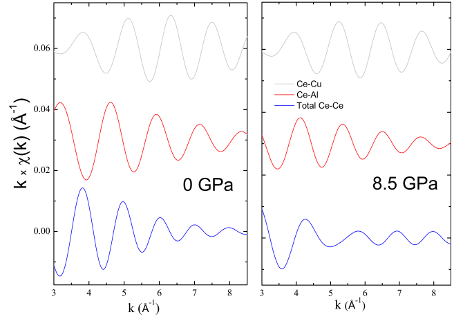
FIG. 5. Separate total Ce-Ce (blue), Ce-Al (red), and Ce-Cu (grey) EXAFS contributions to the total best fit k \times \chi(k) at 0 GPa (left) and 8.5 GPa (right).
