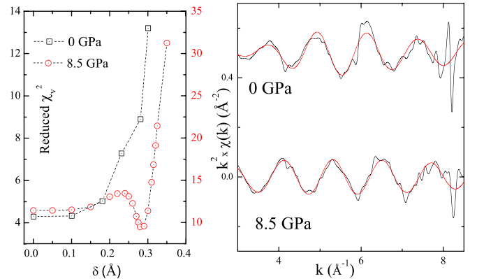
FIG. 4. Left: \chi_v^2 as a function of \delta parameter (splitting of the Ce-Ce distance in \text{Ce}_{60}\text{Al}_{20}\text{Cu}_{20} metallic glass). Right: best fit (red) to EXAFS data k^2 \times \chi(k) (\text{\AA}^{-2}) (black) at 0 GPa (up) and 8.5 GPa (down).
