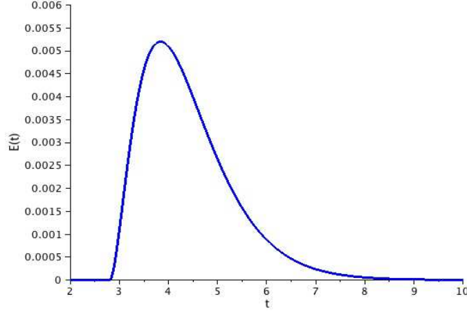
Figure 2: Time evolution of Wooters' concurrence, initial state e_1 \otimes e_1
