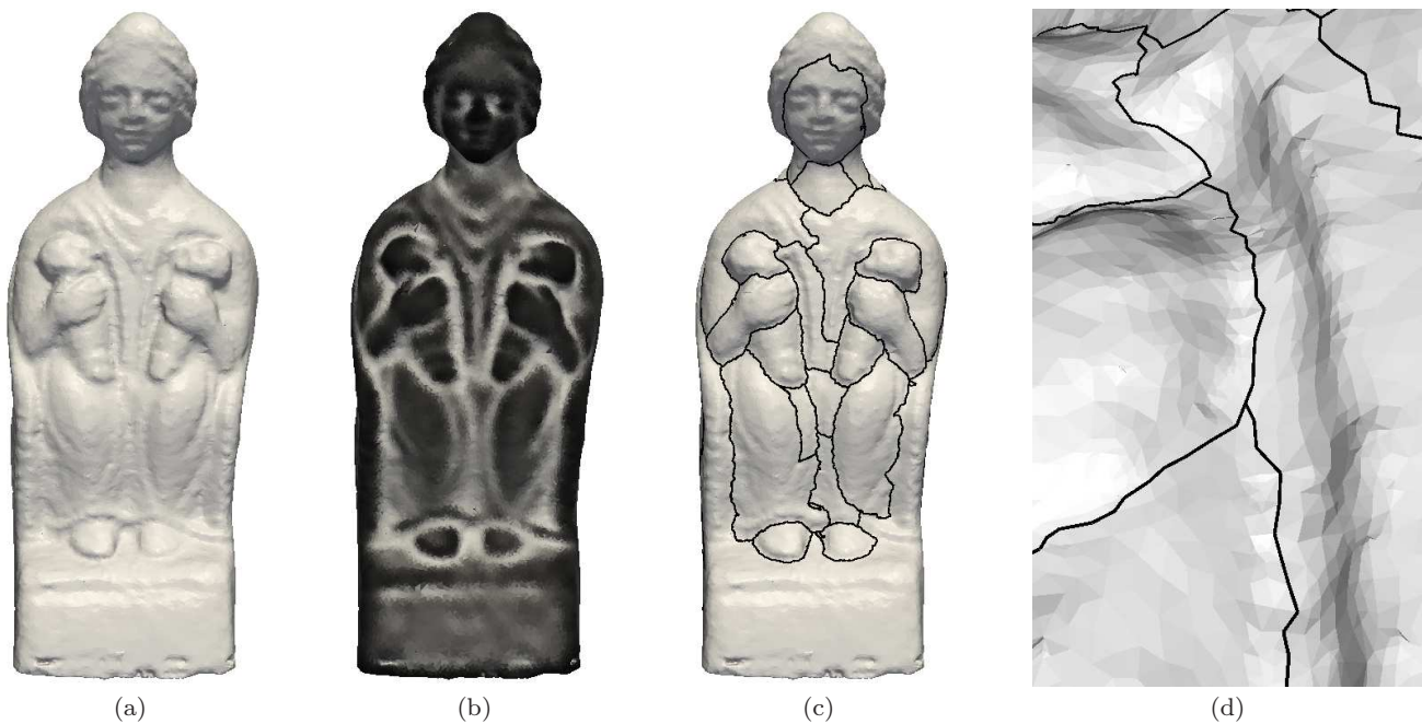
Fig. 6 (a) Rendering of a triangulated surface M . (b) A map F on M (which behaves like the inverse of the mean curvature of the surface, see [44]) (c) A watershed (in black) of F . (d) Zoom on a part of (c). The object M shown in (a) is provided by the French Museum Center for Research.
