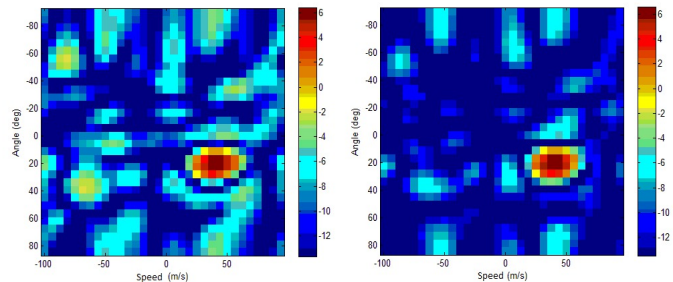
Fig. 4. Filter outputs realized with LR STAP filters built from \hat{\Pi}_c estimated through SCM (left) and the proposed MLE (right).
