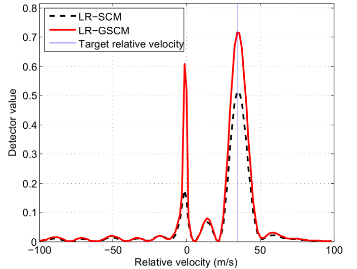
Fig. 3. Value of the LR-SCM and the LR-GSCM detectors for \theta = \theta_d as a function of the relative velocity of the reflector object.
