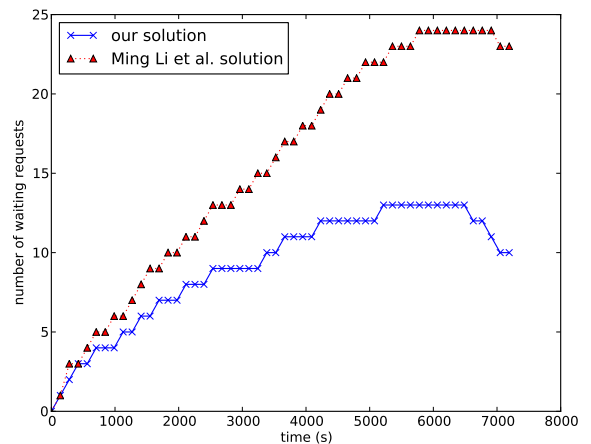
Fig. 5. Performance evaluation with emergency situations
