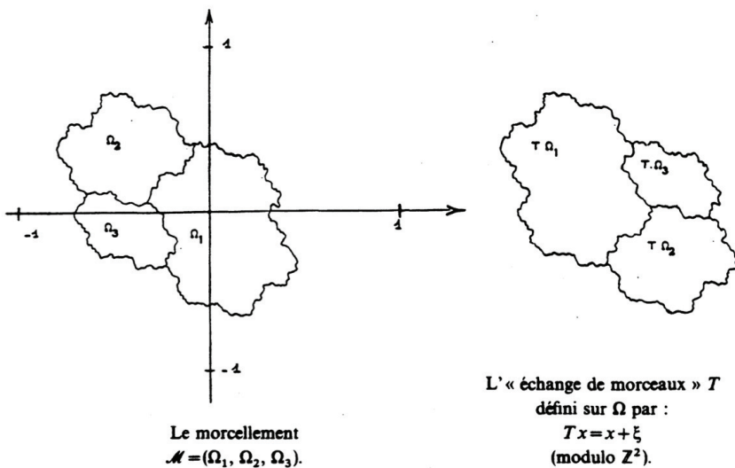
FIGURE 1. The Rauzy splitting (morcellement) associated with the Tribonacci number \theta and the translation T by \xi = (1/\theta, 1/\theta^2) modulo \mathbf{Z}^2 that realizes an exchange of the three pieces \Omega_1, \Omega_2 and \Omega_3 up to their boundaries.
