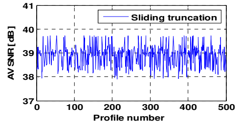
Figure 7. Average global SNR for v = 4 km/h.
