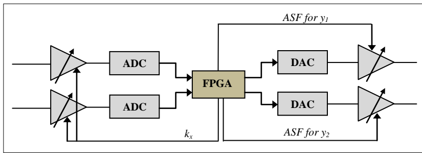
Figure 9. ASF diagram using the gain controlled amplifiers
