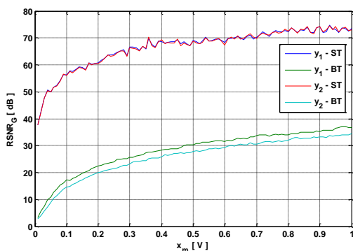
Figure 4. Global SNR versus x_m for TGn model E and 3GPP-LTE model EVA respectively
