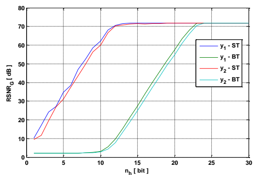
Figure 8. Global output SNR versus n_h for TGn model E and 3GPP-LTE model EVA respectively
