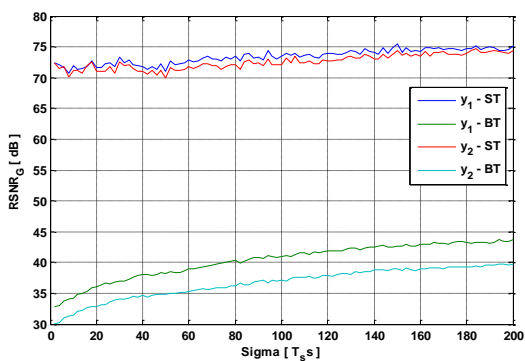
Figure 5. Global SNR versus \Sigma for TGn model E and 3GPP-LTE model EVA respectively
