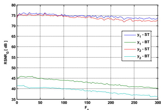
Figure 7. Global output SNR versus F_x for TGn model E and 3GPP-LTE model EVA respectively
