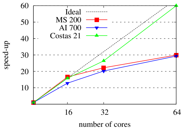
Figure 6. Speed-ups for the three benchmarks problems
