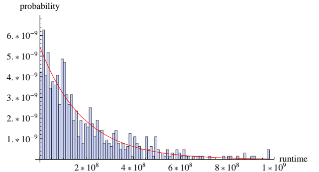
Figure 11. Histogram of the observed number of iterations for 638 runs on the COSTAS ARRAY problem with N = 21 , in blue. In red, the corresponding shifted exponential distribution, statistically estimated.
