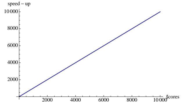
Figure 12. Predicted speed-up for Costas 21.
