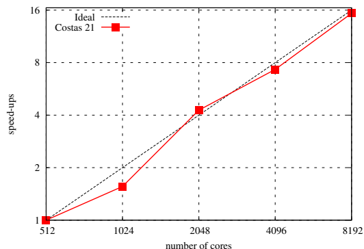
Figure 13. Speed-ups for Costas 21 up to 8,192 cores
