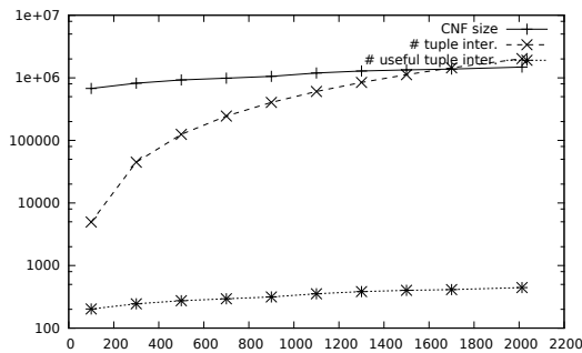
Figure 3. cache influence w.r.t. # tuples in r
