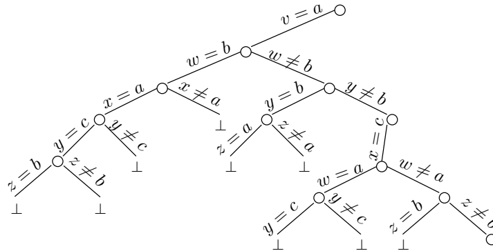
Fig. 1. A partial search tree built by a backtrack search algorithm.
