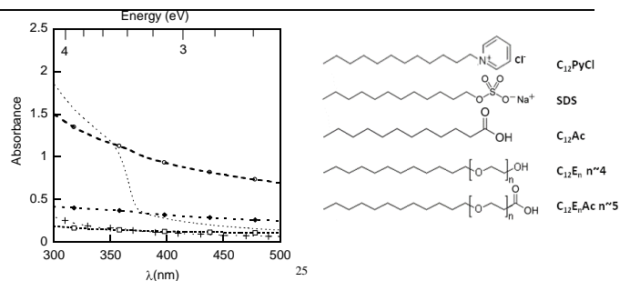
Figure 2 : Absorbance measurements of the aqueous phases after the transfer procedure using C 12 surfactants. (o) C 12 PyCl; (□) lauric acid; (+) C 12 E 4 ; (◆) SDS; (...)Lauryl-5. Surfactant concentration: 3mM.
