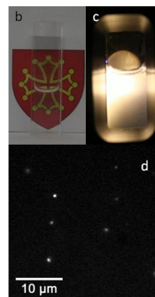
Figure 7 : (a) Absorbance and emission spectra of ZnO Ncs in dichloromethane and after transfer to water using Oleyl-10, 3 mM. Red line: Spectra in dichloromethane. Blue line: spectra in water after transfer. (b) Photograph of the transparent ZnO Ncs aqueous solution after transfer. (c) Photograph of the ZnO Ncs aqueous solution under irradiation at \lambda_{\text{exc}} = 360 nm. (d) Fluorescence microscopy image of ZnO Ncs in an aqueous buffer solution (Tris).
