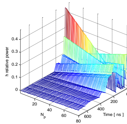
Figure 3. Switching between E_2 and E_3
