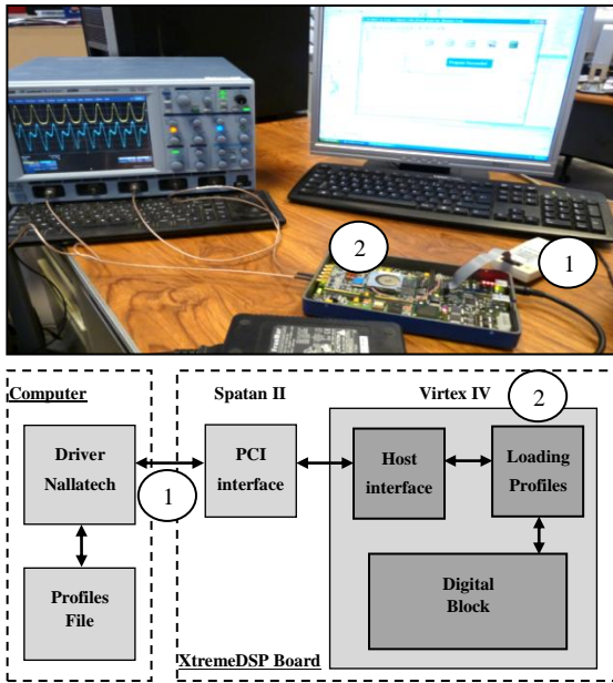
Figure 5. Connection between the computer and the XtremeDSP board.
