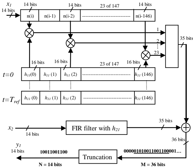
Figure 4. FIR 147 with 23 multipliers for one h_{11} and h_{21}
