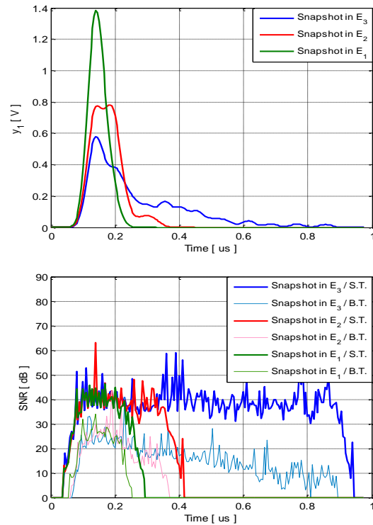
Figure 6. Three Snapshots of y_1 in E_1 , E_2 and E_3 respectively with their SNR.
