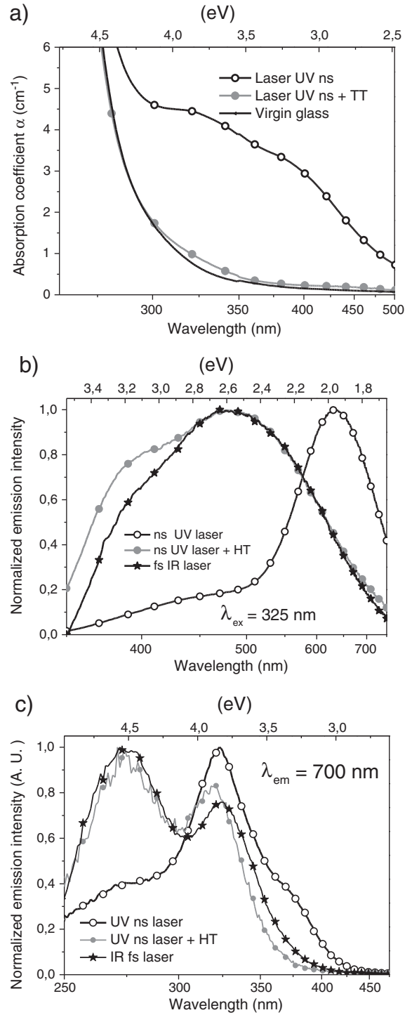
Fig. 3. a) Absorption spectra before, after ns-laser irradiation and after heat treatment ( 400^\circ\text{C} , 10 min), b) emission spectra for \lambda_{\text{exc}} = 325 \text{ nm} , and c) excitation spectra at \lambda_{\text{em}} = 700 \text{ nm} after ns-laser irradiation, after ns laser irradiation and heat treatment and after fs-laser irradiation.
