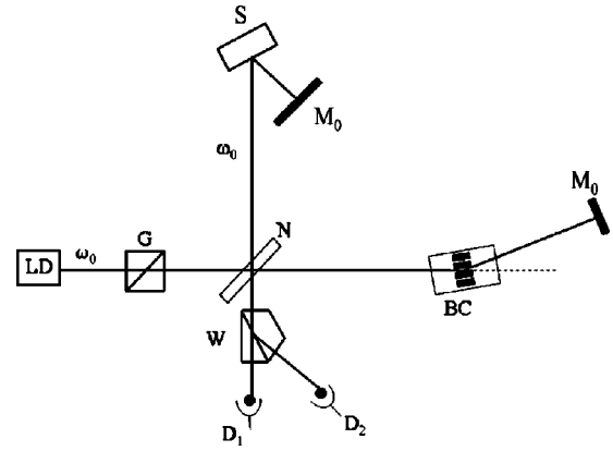
FIG. 1. The setup of the Hazebroek and Holscher interferometric ellipsometer with a Bragg cell. BC: Bragg cell, D: photodiodes, G: Glan–Thomson polarizer, LD: laser diode, M_0 : mirror, N: neutral density beam splitter, S: sample, and W: Wollaston prism.
