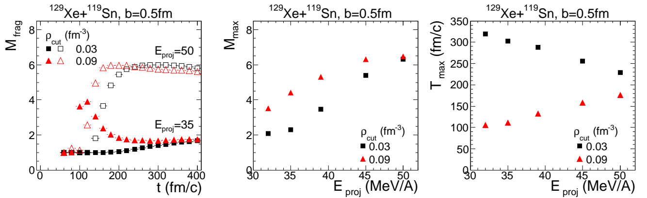
FIG. 2: Left panel : multiplicity of fragments ( M_{frag} ) time evolution for two density cut-off (black squares and red triangles respectively for \rho_{cut}=0.03 and 0.09 \text{ fm}^{-3} ) and for two bombarding energies (full and open symbol respectively for E_{proj}=35 and 50 \text{ MeV/A} .); middle panel : Evolution with bombarding energies of the maximum value ( M_{max} ) reached by multiplicity of fragment for the two density cut-off; right panel : evolution with bombarding energies of time ( T_{max} ) when maximum of fragment multiplicities is reached for the two density cut-off.
