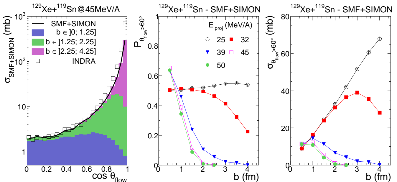
FIG. 3: Left panel : distributions in mb of the flow angle cosine ( \cos \theta_{flow} ) distribution : black line distribution is for SMF+SIMON events and the three colors stand for the relative contribution of 3 impact parameter ( b ) ranges. Black squares distribution is for INDRA data after normalization to the simulated cross section (see text for details); middle panel : probability for each impact parameter ( b ) that simulation events fulfil the condition \theta_{flow} > 60^\circ ; right panel : cross section contribution of each impact parameter to the selected sample of events.
