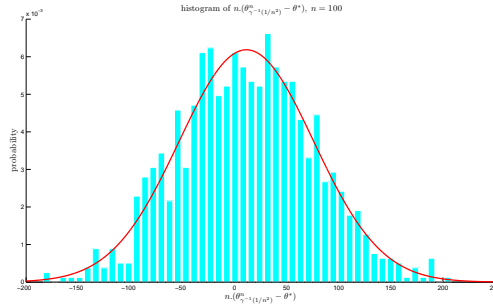
FIGURE 2. Histogram of n(\theta_{\gamma^{-1}(1/n^2)}^n - \theta^*) , n = 100 , with N = 1000 samples.
