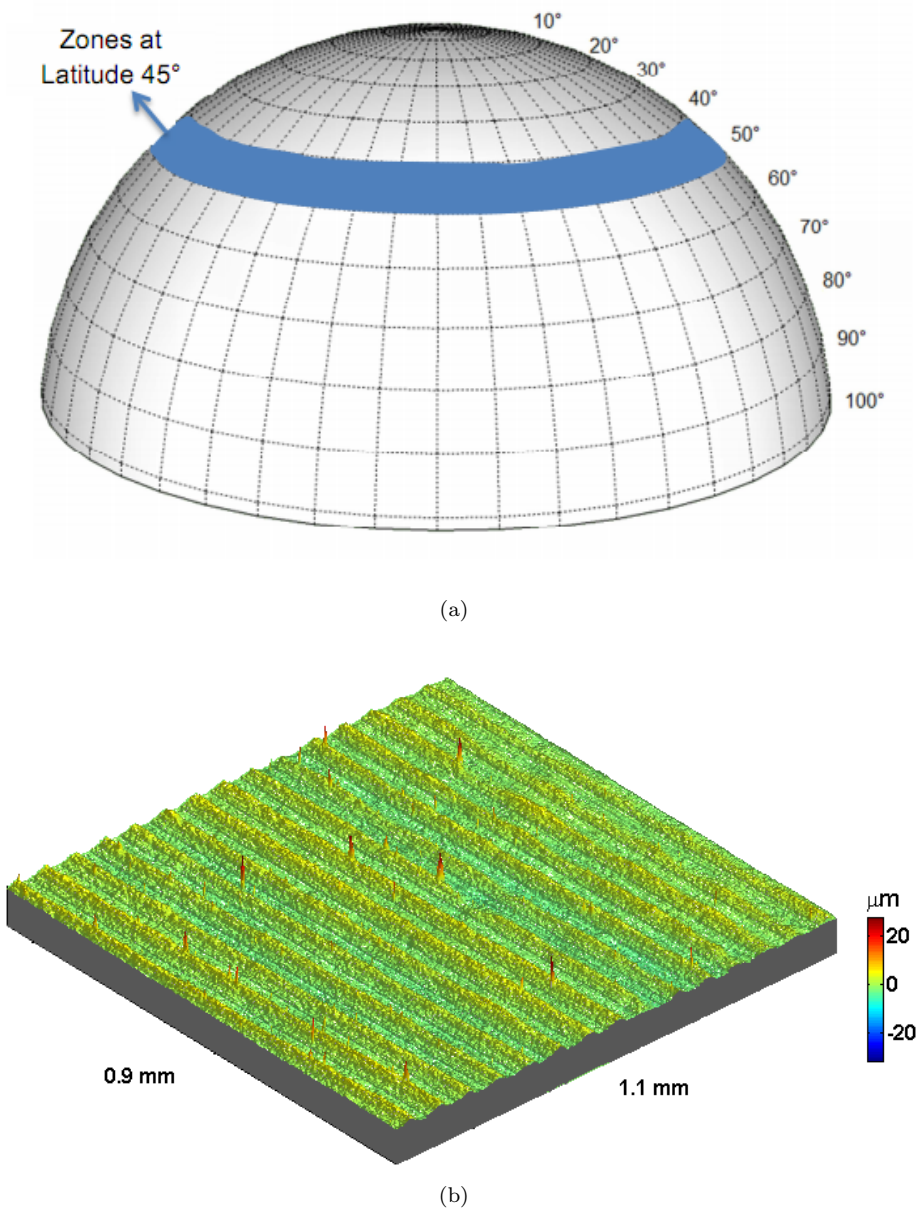
Figure 3: (a). A synthetic 3D-dimensional model of the UHMWPE dual mobility cup. The blue colored zone refers to the latitude 45°. (b) A 3D height map measured from a local region, at the 45° latitude on a maximum area of 1.1 \times 0.9 \text{ mm}^2
