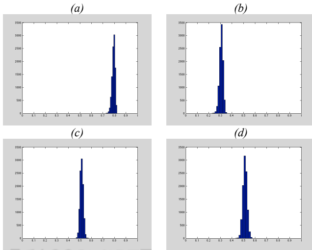
Figure 13: Histograms of W_k^u for the event 74 (a), 26 (b), 41 (c), 33 (d).
