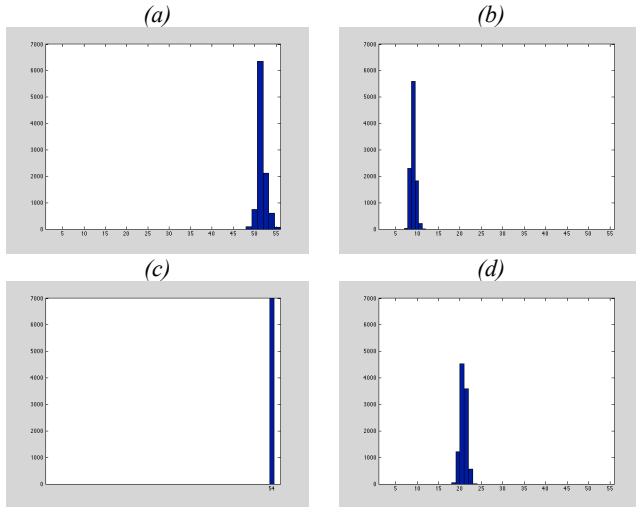
Figure 12: Histograms of RUL_k^u for the event 74 (a), 26 (b), 41 (c), 33 (d).
