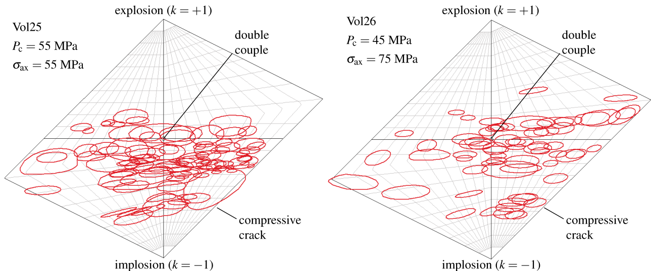
Figure 10. Focal mechanisms for (left) 95 AEs from experiment Vol25 and (right) 65 AEs from experiment Vol26 in a T-k plot [Hudson et al., 1989]. The size of the red ellipsoids corresponds to the uncertainties.
