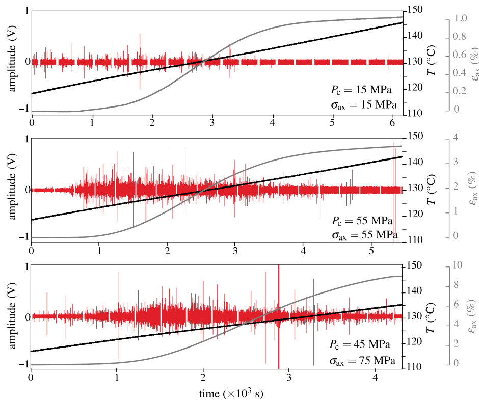
Figure 7. Continuous acoustic waveforms (red), temperature (black line), and axial shortening (gray line) during dehydration tests. White spaces within the waveforms corresponds to active wave velocity surveys. The dehydration reaction, which starts just above 120°C, corresponds to a swarm in acoustic emission (AE) activity.
