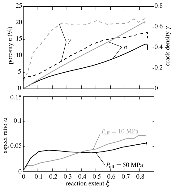
Figure 12. Evolution of (top) porosity and crack density and (bottom) aspect ratio during dehydration in a hydrostatic stress state. Porosity is calculated from equation (B4); crack density is calculated from equation (8). Aspect ratio results from the inversion procedure are detailed in Appendix B.
