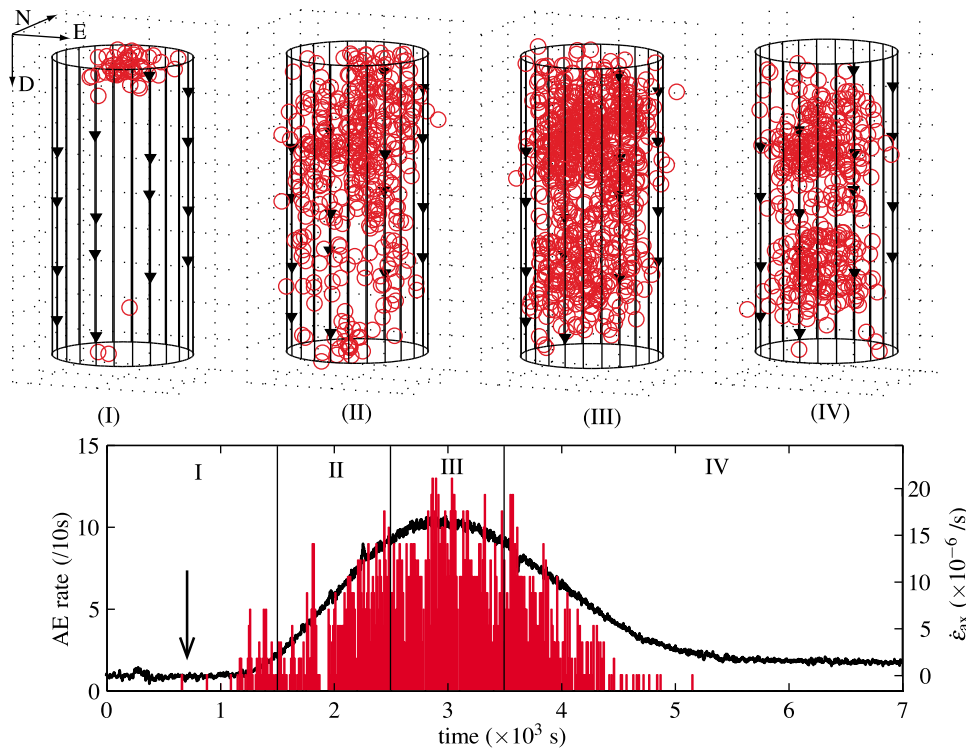
Figure 8. Spatiotemporal distribution of AEs, AE rate, and shortening rate during the test performed at P_c = \sigma_{ax} = 55 MPa. AEs occurring during phase I are localized at the top end of the sample, close to the pore fluid outlet. AEs are then more homogeneously distributed throughout the sample (phases II–IV). AE activity stops concomitantly with axial shortening. The arrow indicates the onset of wave velocity decrease.
