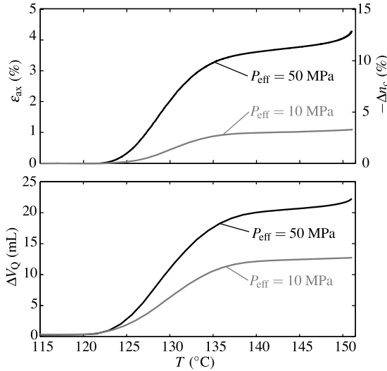
Figure 2. Shortening, compaction, and fluid release during drained hydrostatic heating tests.
