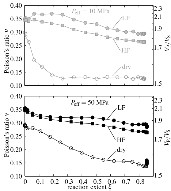
Figure 13. Poisson's ratio evolution during dehydration extrapolated to low-frequency waves using the differential effective medium (DEM) model (see section 4.1.2). HF, high frequency; LF, low-frequency bound, computed using Gassmann theory; dry, dry (or, equivalently, drained) result using the DEM model in absence of fluid.
