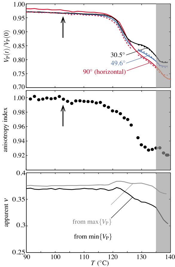
Figure 14. (top) Normalized, average P wave speeds in the three available orientations and (middle) anisotropy index evolution during the test performed at P_c = 45 MPa and \sigma_{ax} = 75 MPa. (bottom) Two apparent Poisson's ratios calculated from the fastest (gray line) and the slowest (black line) P wave speeds measured during the test. The shaded area corresponds to the stroke end of the piston and should not be interpreted. Solid lines denote averaged, normalized data. Dashed lines denote fitted velocities using equation (10). Arrow indicates the loading up to the target value of \sigma_{ax} .
