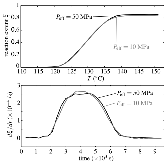
Figure 3. Reaction progress and reaction rate as a function of temperature and time during hydrostatic drained tests. The reaction progress is calculated from porosity compaction and fluid release, using equation (4).
