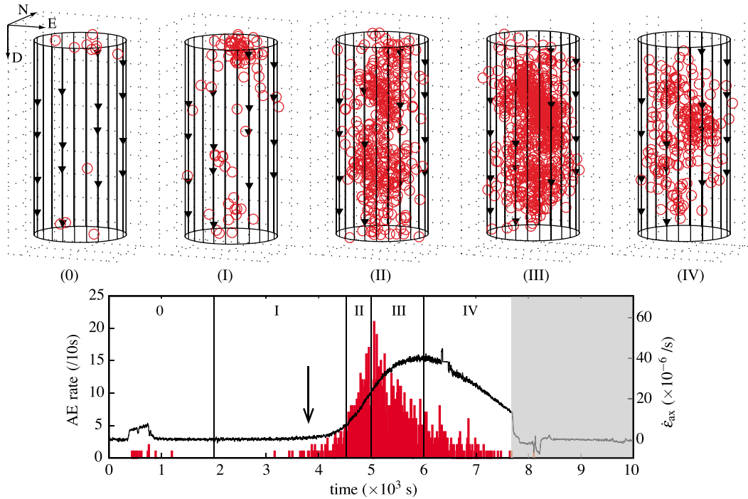
Figure 9. Spatiotemporal distribution of AEs, AE rate, and shortening rate during the test performed at P_c = 55 MPa and \sigma_{ax} = 75 MPa. Phase 0 corresponds to the axial loading up to the target axial stress; no significant AE activity is recorded during this step. AEs occurring during phase I are localized at the top end of the sample, close to the pore fluid outlet. AEs are then more homogeneously distributed throughout the sample (phases II–IV). AE activity stops concomitantly with axial shortening. The arrow indicates the onset of wave velocity decrease. The shaded area corresponds to the end stroke of the piston.
