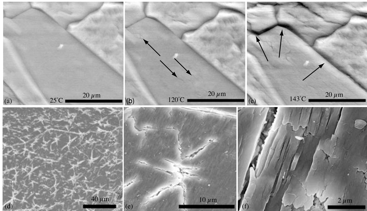
Figure 11. Microstructure evolution (a–c) during and (d–f) after dehydration. Secondary electron mode. Figures 11a–11c were taken in situ, without coating, at 360 Pa chamber pressure. At around 120°C, intragranular cracks appear and grow. Then, grain boundaries progressively open. Figures 11d–11f were taken on the same sample, after carbon coating, in a FE-SEM under an accelerating voltage of 10 kV. Orientations of intragranular cracks are not random and are likely to be dictated by the crystal orientation of initial gypsum grains [Sipple et al. , 2001].
