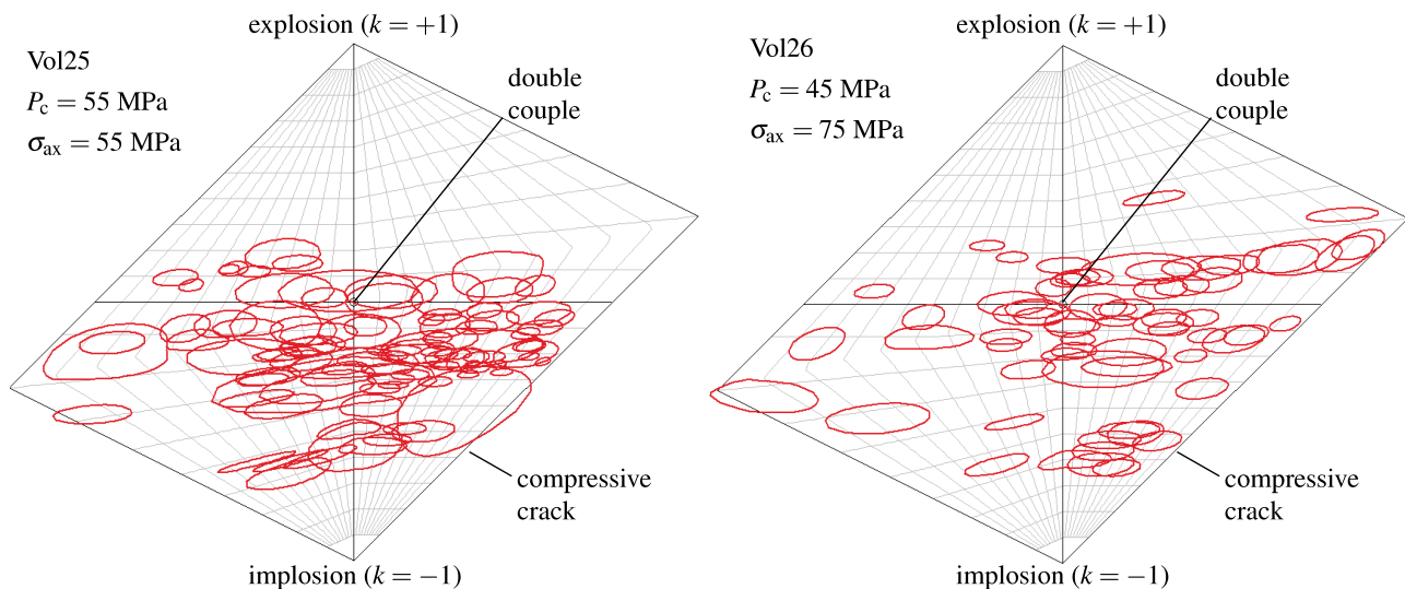
Figure 10. Focal mechanisms for (left) 95 AEs from experiment Vol25 and (right) 65 AEs from experiment Vol26 in a T-k plot [Hudson et al., 1989]. The size of the red ellipsoids corresponds to the uncertainties.
