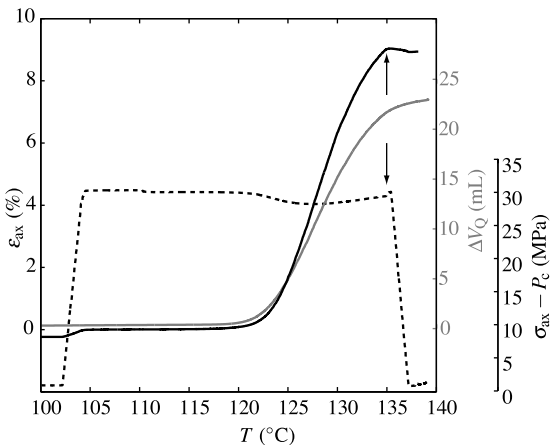
Figure 4. Shortening (solid black line), fluid release (solid gray line) and differential stress (dashed line) during the drained heating test performed in creep conditions at P_c = 45 MPa and \sigma_{\text{ax}} = 75 MPa. The arrows indicate the piston stroke end.
