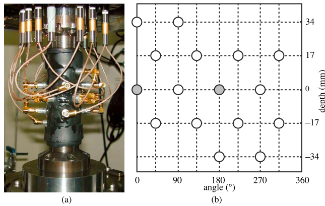
Figure 1. (a) Photograph of the sample assembly and (b) sensor map. The white circles correspond to P wave transducers, and the gray circles are S_h wave transducers.
