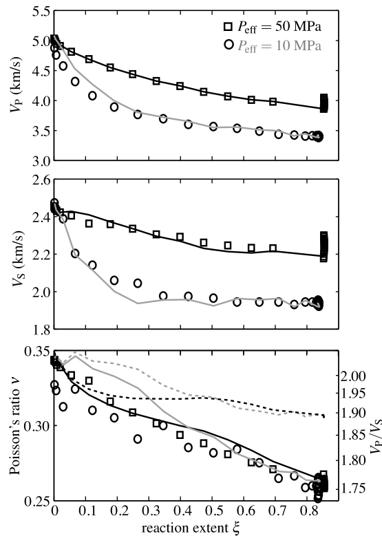
Figure 6. P and S wave speeds and Poisson's ratio during dehydration. Measurements are performed using a single pair of sensors along a horizontal path. Solid black and gray lines correspond to simulations calculated using the effective medium model presented in section 4.1. Dashed lines correspond to a calculated Poisson's ratio that does not account for changes in elastic moduli of the solid skeleton (see section 4.1 for details).
