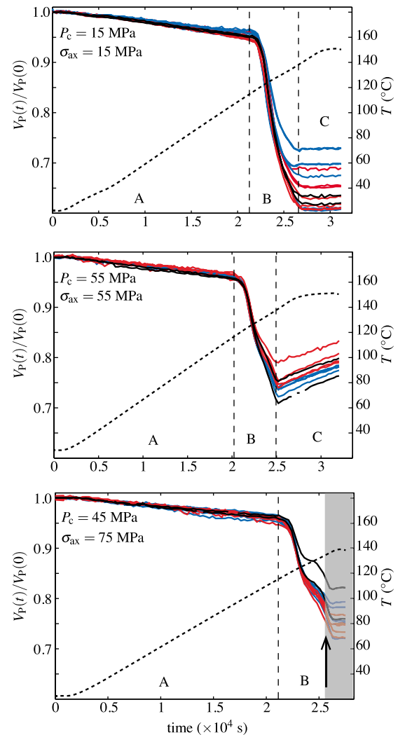
Figure 5. Relative evolution of P wave velocity during dehydration tests. The wave speeds are normalized by their initial value, measured at room temperature and under the stress conditions denoted in the graphs. Temperature is indicated by the dotted line. Black lines denote measurements along raypaths oriented at 30.5^\circ from the vertical. Blue lines correspond to raypaths oriented at 49.6^\circ from the vertical. Red lines correspond to horizontal raypaths. Arrow and gray area in the bottom graph denote the onset of the piston stroke end. Three steps are distinguished. During phase A, V_p decreases slowly and homogeneously in the samples. During phase B, dramatic and heterogeneous decreases in V_p are recorded. During phase C, P wave velocities slowly increase.
