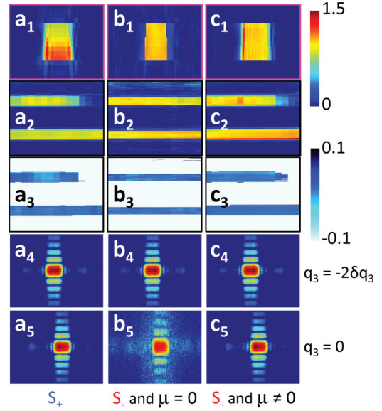
FIG. 3. (Color online) Regularization on numerical data. (a) Same as Fig. 2(b) for the reconstructed object obtained from the S_+ data set. (b) Same as (a) for the reconstructed object obtained from the undersampled data set S_- . (c) Same as (b) introducing the regularization based on the support of the sample.
