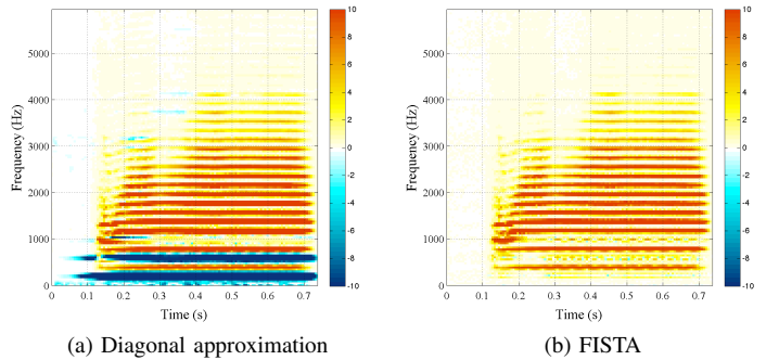
Figure 5: Gabor masks obtained for \mu = 10^{-3} , d = \|\boldsymbol{\sigma} - 1\|_2^2 .
