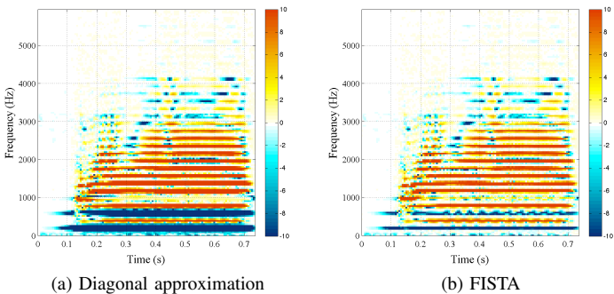
Figure 4: Gabor masks obtained for \mu = 10^{-3} , d = \|\boldsymbol{\sigma} - 1\|_2^2 .
